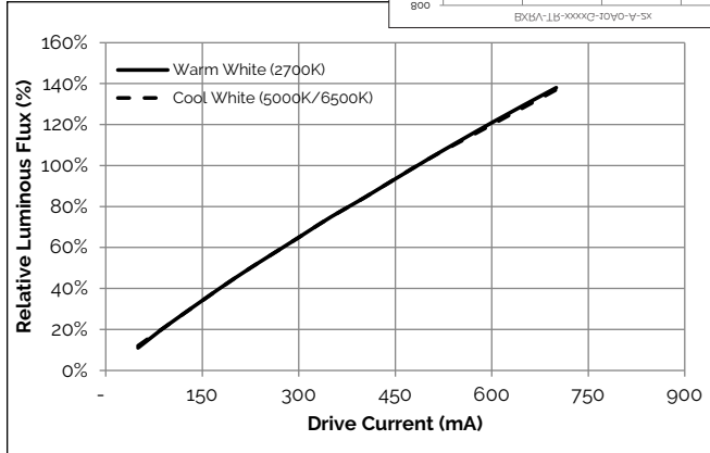
Figure 8: Relative Flux vs. Drive Current, T_c = 25^\circ\text{C}
