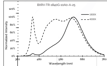
Figure 35: 1800K - 4000K with 90 CRI
