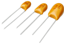
CA42: Radial Epoxy Dipped
