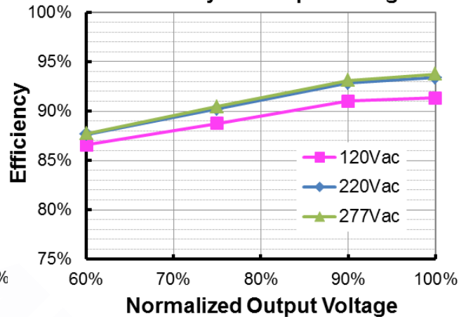
EUM-150S150Lx ( I_o=1500mA ) Efficiency vs. Output Voltage
