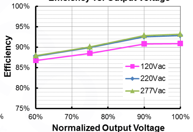
EUM-150S210Lx ( I_o=2100mA ) Efficiency vs. Output Voltage
