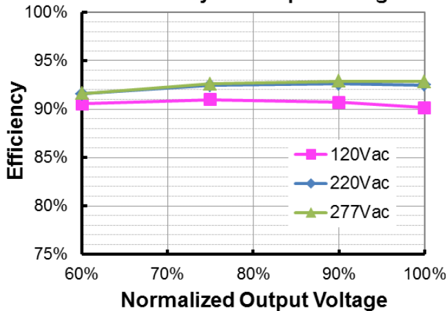
EUM-150S210Lx ( I_o=1400mA ) Efficiency vs. Output Voltage
