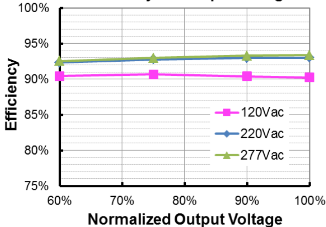
EUM-240S350Lx ( I_o=2150mA ) Efficiency vs. Output Voltage
