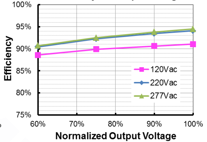
EUM-240S150Lx ( I_o=1500mA ) Efficiency vs. Output Voltage
