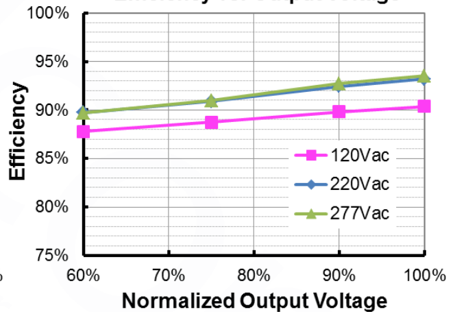
EUM-240S350Lx ( I_o=3500mA ) Efficiency vs. Output Voltage
