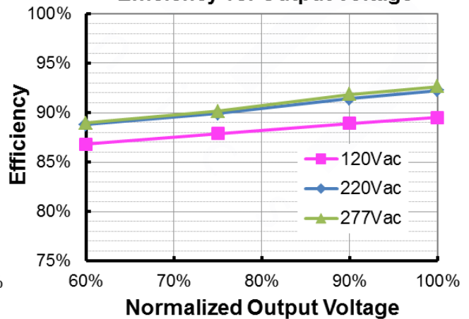
EUM-240S350Lx ( I_o=3500mA ) Efficiency vs. Output Voltage
